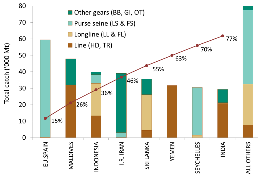
Fig. 2. Yellowfin tuna: average catches in the Indian Ocean over the period 2012–15, by country. Countries are ordered from left to right, according to the importance of catches of yellowfin reported. The red line indicates the (cumulative) proportion of catches of yellowfin for the countries concerned, over the total combined catches of this species reported from all countries and fisheries. Data as of September 2016.
