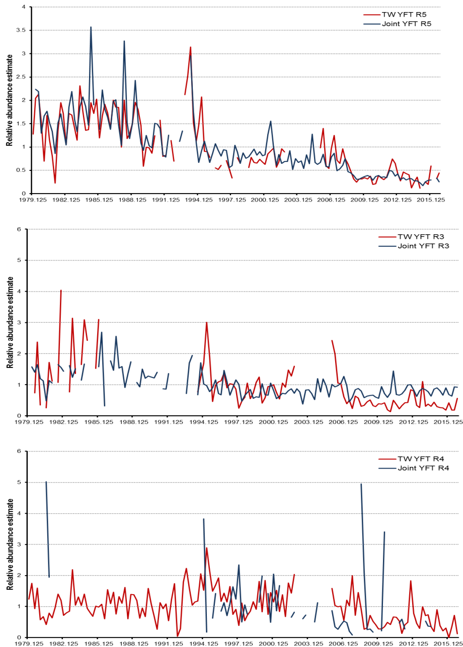
Fig.13. Comparisons of Taiwan,China yellowfin tuna CPUE time series (red) with those estimated during the 2016 collaborative project (blue) by region.
