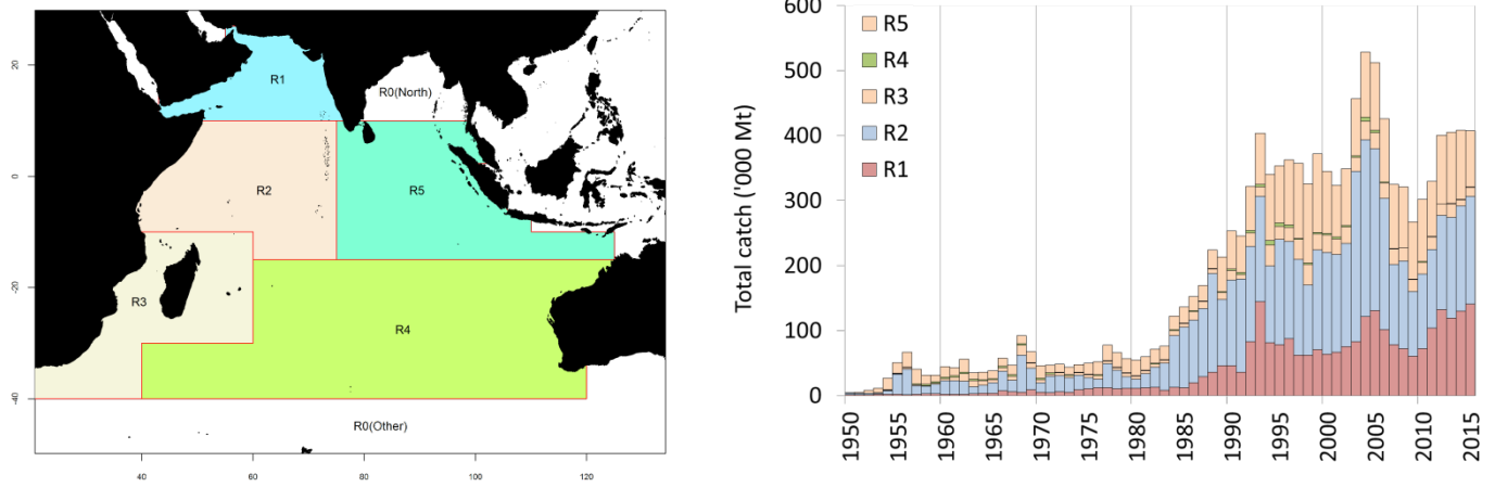
Fig. 3(a-b). Yellowfin tuna: Catches of yellowfin tuna by area by year estimated for the WPTT (1950–2015). Catches in areas R0 were assigned to the closest neighbouring area for the assessment. Data as of September 2016.
