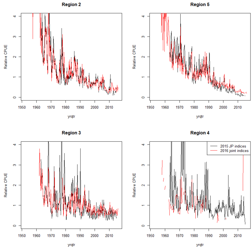
Fig.12: Comparison of the 2016 joint indices described in this paper (red) with the Japanese indices developed in 2015 and used in the 2015 yellowfin stock assessment (black).
