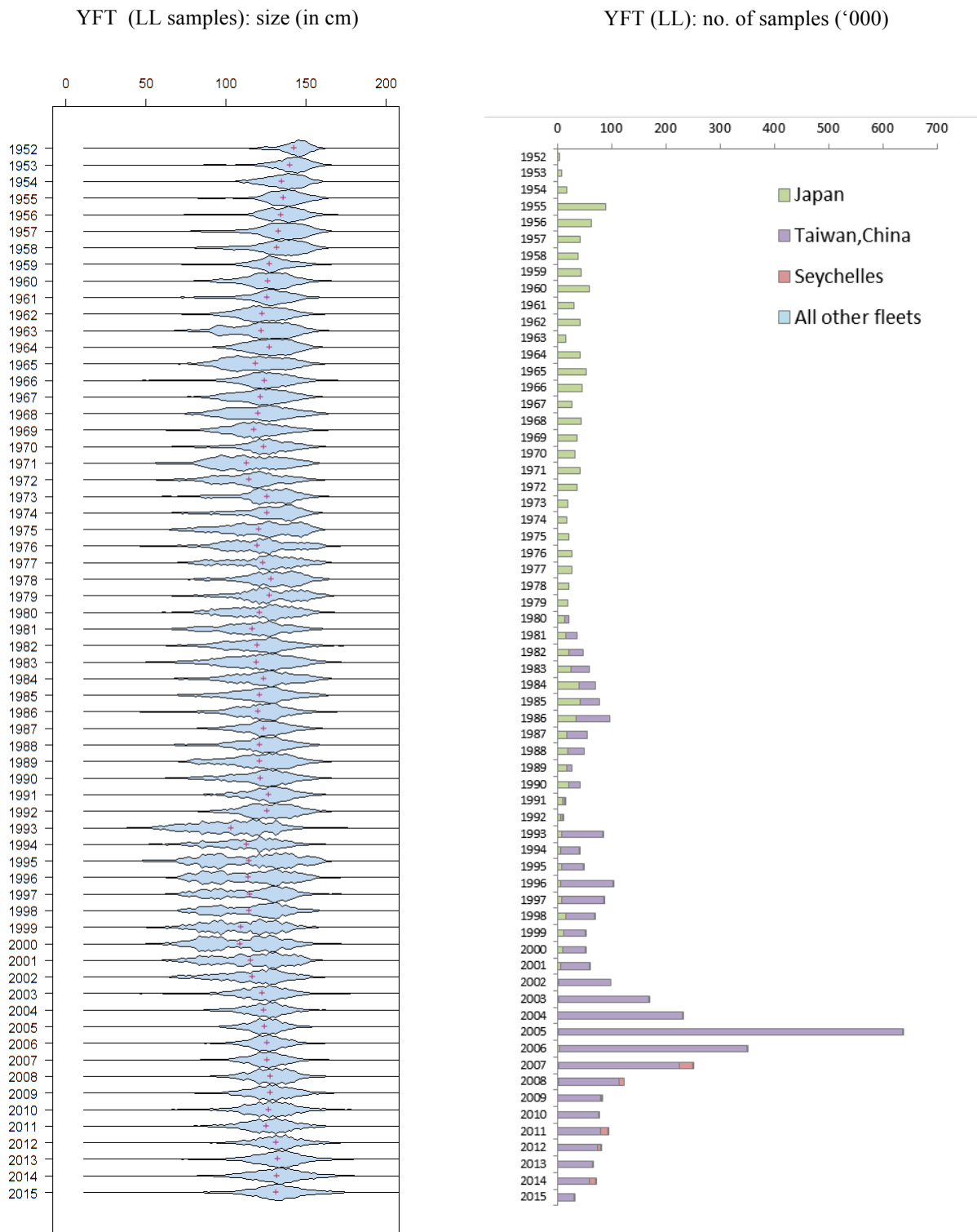
Fig. 8 Yellowfin tuna (longline): Left: length frequency distributions for longline fisheries (total amount of fish measured by 2 cm length class) derived from data available at the IOTC Secretariat. Right: Number of yellowfin tuna specimens sampled for lengths, by fleet (longline only).
