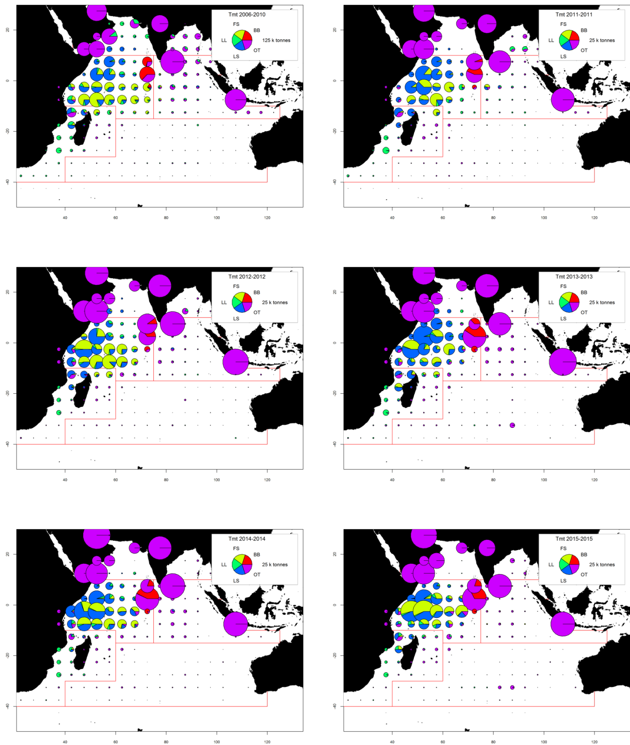
Fig. 4(a-f). Time-area catches (total combined in tonnes) of yellowfin tuna estimated for the period 2006–2010 by type of gear and for 2011–2015, by year and type of gear. Longline (LL), Purse seine free-schools (FS), Purse seine associated-schools (LS), pole-and-line (BB), and other fleets (OT), including drifting gillnets, and various coastal fisheries.
