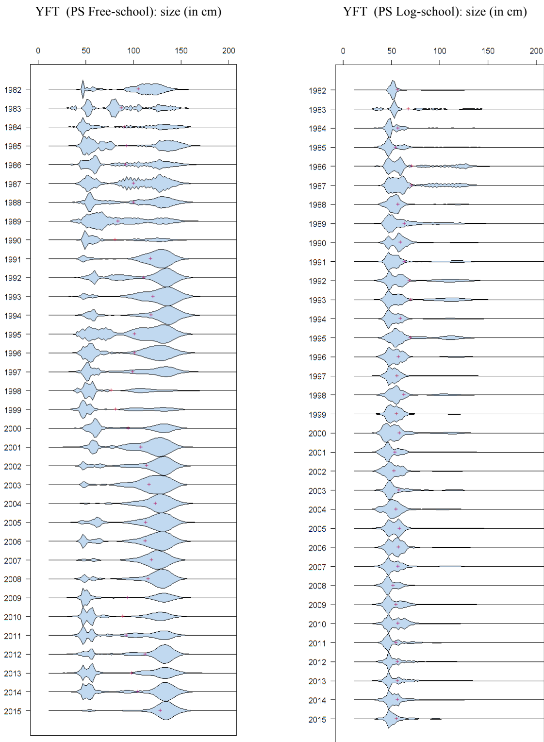
Fig.7 Yellowfin tuna (purse seine): Left: length frequency distributions for YFT PS Free school fisheries (by 2 cm length class). Right: Length frequency distributions for YFT PS Associated (log) school fisheries (by 2 cm length class). Source: IOTC database.
